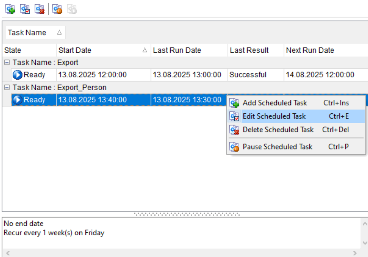
Task Scheduler
