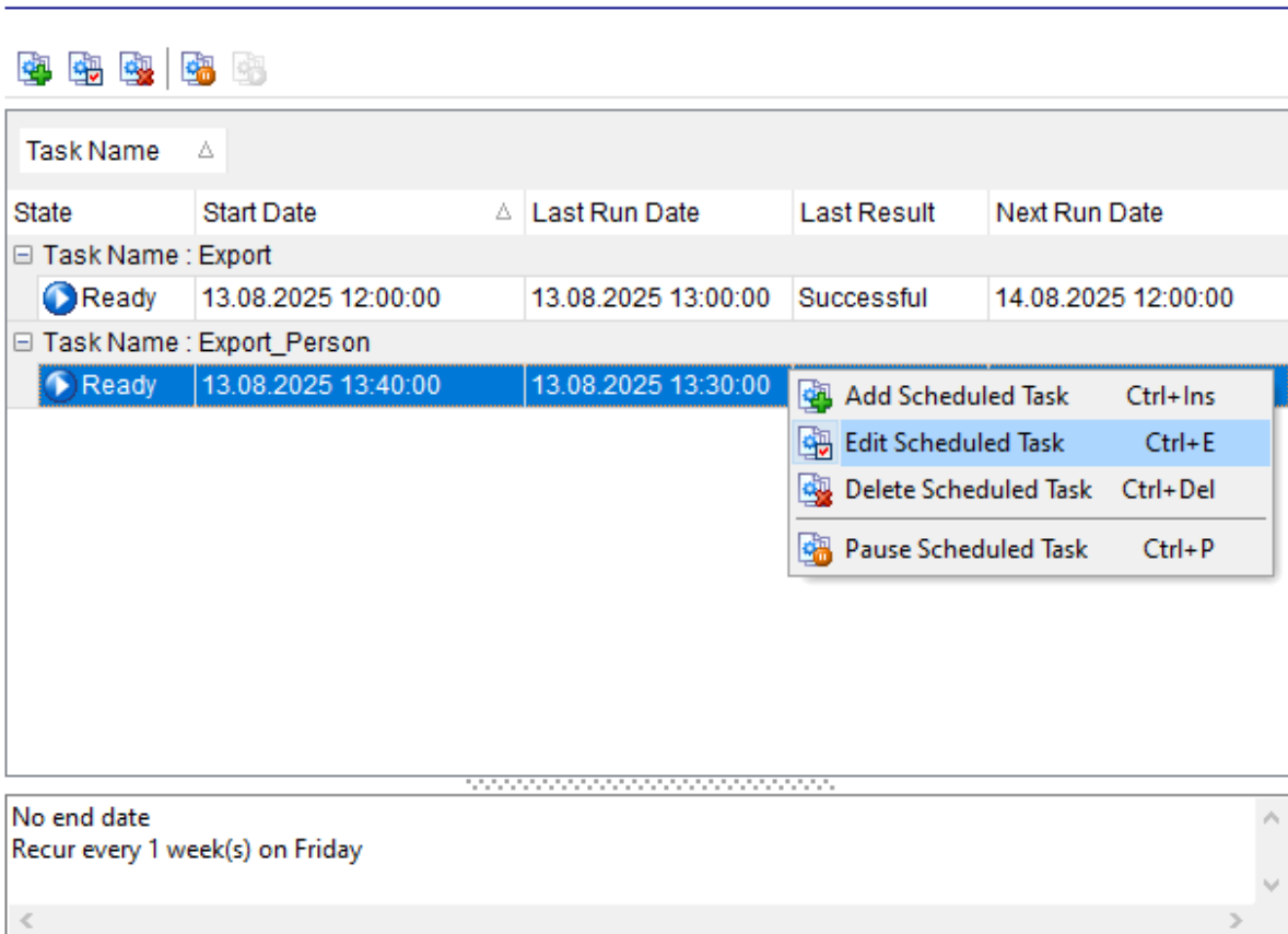
Task Scheduler
